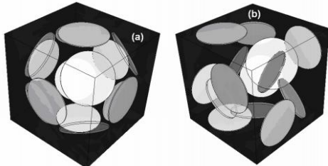
Figure 8: Cell (a) and Dispersed (b) RVE geometries (11 platelets of aspect ratio 30) ;
