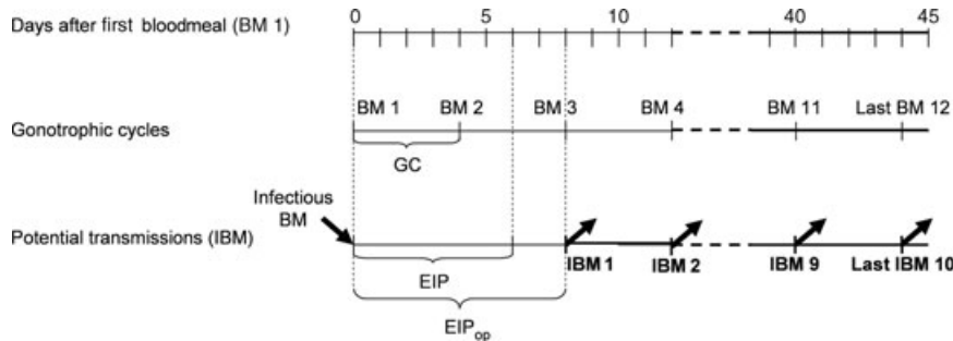
Fig. 1. Diagram of variables used in the model. In this example, the infectious bloodmeal ( \searrow , transmits pathogen to the mosquito) is the first bloodmeal taken by the mosquito, the maximum longevity of a mosquito = 45 days, the gonotrophic cycle duration = 4 days, the extrinsic incubation period (EIP) = 6 days, and the operational EIP ( EIP_{op} ) = 8 days (i.e. = 2 GC). BM, bloodmeal; GC, gonotrophic cycle; IB, infective bite; IBM, infectious bloodmeal; ( \nearrow , transmits pathogen to host); bold text indicates the period during which a mosquito can potentially transmit the dengue virus.
