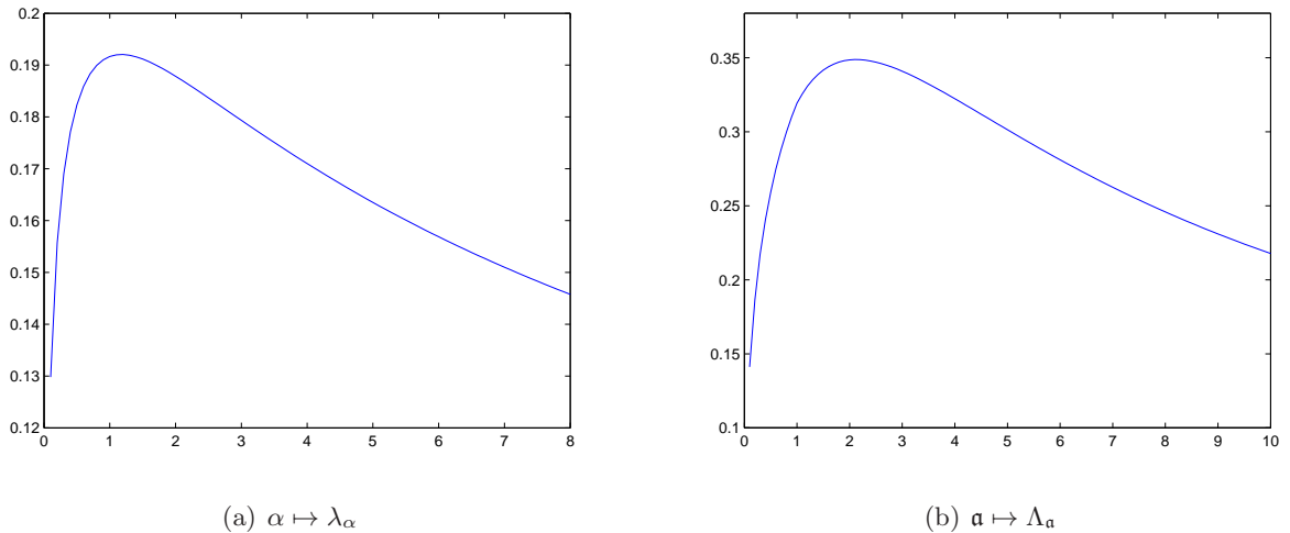
Figure 2: The dependences of the first eigenvalue on polymerization and fragmentation parameters for coefficients which satisfy the assumptions of Theorem 1 are plotted. The coefficients are chosen to obtain non monotonic functions. 2(a): \tau(x) = \frac{8x^{0.2}}{1+2x^{4.2}} , \beta(x) = \frac{x^3}{15+x^{4.5}} and \kappa(x, y) = \frac{1}{y} \mathbb{1}_{0 \leq x \leq y} . We have \lim_{x \rightarrow 0} \beta(x) = \lim_{x \rightarrow \infty} \beta(x) = 0 , so \lim_{\alpha \rightarrow 0} \lambda_\alpha = \lim_{\alpha \rightarrow \infty} \lambda_\alpha = 0 . 2(b): \tau(x) = \frac{1.2x^{1.8}}{1+2x^{2.8}} , \beta(x) = \frac{4x^2}{10+x^{0.8}} and \kappa(x, y) = \frac{1}{y} \mathbb{1}_{0 \leq x \leq y} . We have \lim_{x \rightarrow 0} \frac{\tau(x)}{x} = \lim_{x \rightarrow \infty} \frac{\tau(x)}{x} = 0 , so \lim_{\mathbf{a} \rightarrow 0} \Lambda_{\mathbf{a}} = \lim_{\mathbf{a} \rightarrow \infty} \Lambda_{\mathbf{a}} = 0 .
