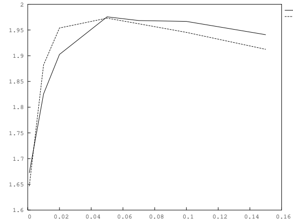
Fig. 14. Comparison of U(x) and N(x) for the (1+1)ES) with adapted mutation radius, in 10 generations. Mean best fitness (ordinate) vs mean mutation radius (abscissa).
