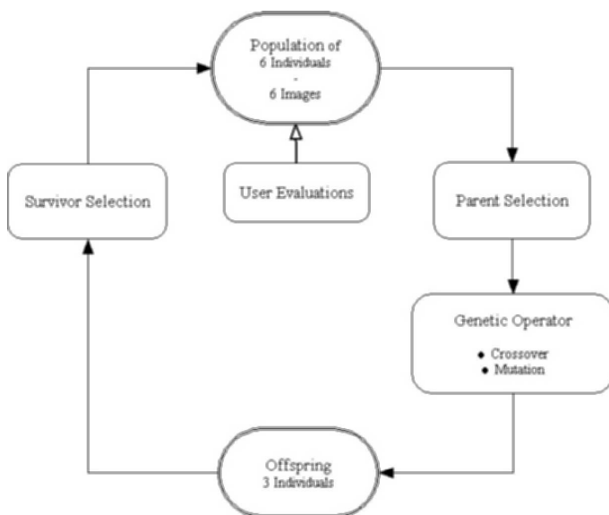
Figure 12.4. The small population denoising IEA genetic engine.
