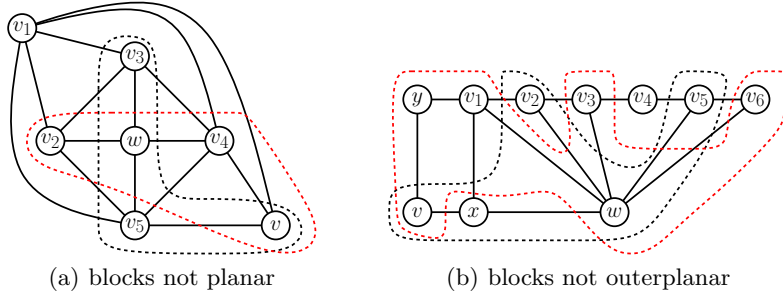
Fig. 3. Illustration of some examples. Solid edges indicate a support, dashed curves indicate hyperedges that contain more than two vertices.
