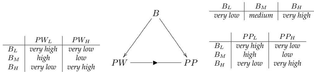
Figure 5.7: A user preference example using LCP-nets.
