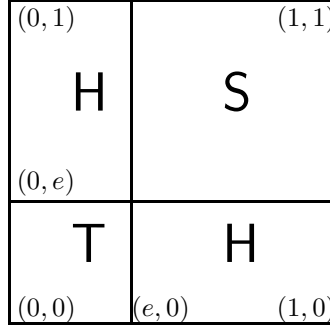
Figure 2: The representation of a uninorm from Proposition 19
