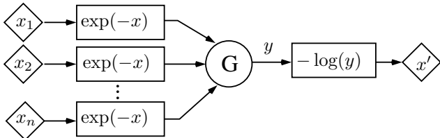
Fig. 3: Principle of exponential-domain computation.
