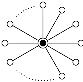
Figure 1: Brauer tree of D \rtimes E
