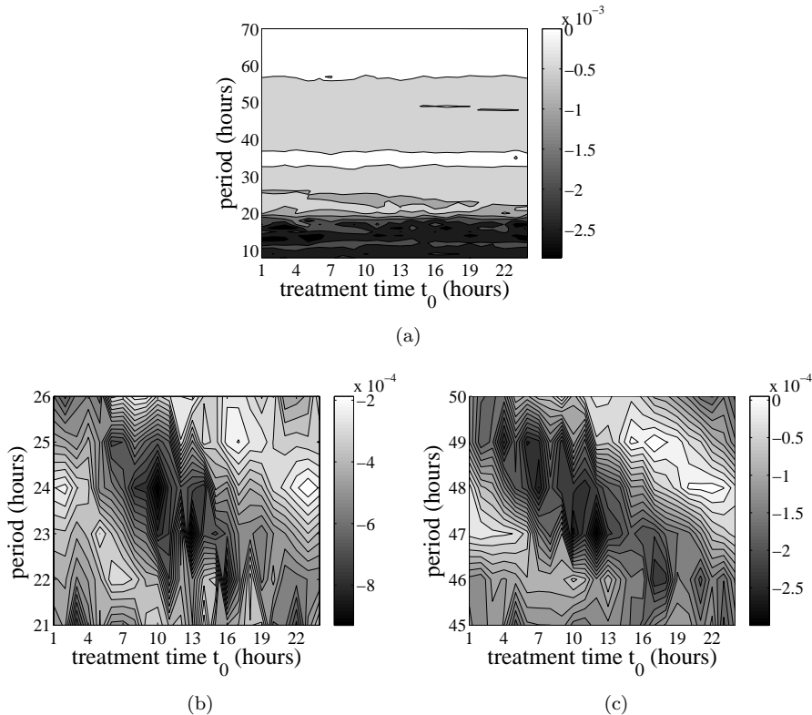
FIG. 3.4. Treatment outcomes for normal cells ( c_x = 0.5 ). The gray scale shows the value of \lambda as a function of the first day delivery time t_0 and the interval T between two consecutive drug administrations. (a) Growth exponent \lambda for t_0 ranging from 1 a.m. to midnight, and T ranging between 8 and 65 hours. (b) Specific region around period T=24 hours. (c) Specific region around period T=48 hours, respectively. All three panels correspond to the same numerical simulations. Low values of \lambda indicate bad treatment outcomes (high toxicity, dark regions) and high values indicate good treatment outcome (low toxicity, light regions).
