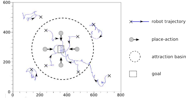
Fig. 4. Trajectories of the robot. Place-action associations are learned 0.8 meter from the goal and the attraction basin is approximately 4 meters wide. When the robot is inside its attraction basins, it successfully navigates toward its goal. Outside the attraction basin the robot is lost. Even with this raw strategy, the robot sometimes reaches the attraction basin (by mere chance) and then converges toward its goal. These trajectories are obtained via infra red video tracking.
