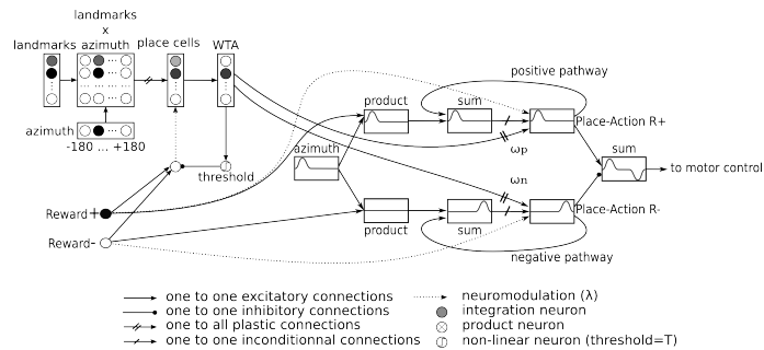
Fig. 3. Sensorimotor visual navigation : a visual place cell is constructed from recognition of a specific landmarks-azimuths pattern and an action (a direction) is associated to it. When one neuron of the Place-Action group receives a neuromodulation from the reward (positive reward in this example), it learns the association between the current robot location and its direction. The positive conditioning group activates the learned direction while the negative conditioning inhibits the learned direction.
