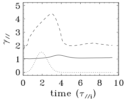
Figure 14. Parallel sheath transmission coefficients for the ions (solid line) and the electrons (dashed line), for a case with time-distributed source. The dotted lines represent the source temporal profile g(t) , in arbitrary units.
