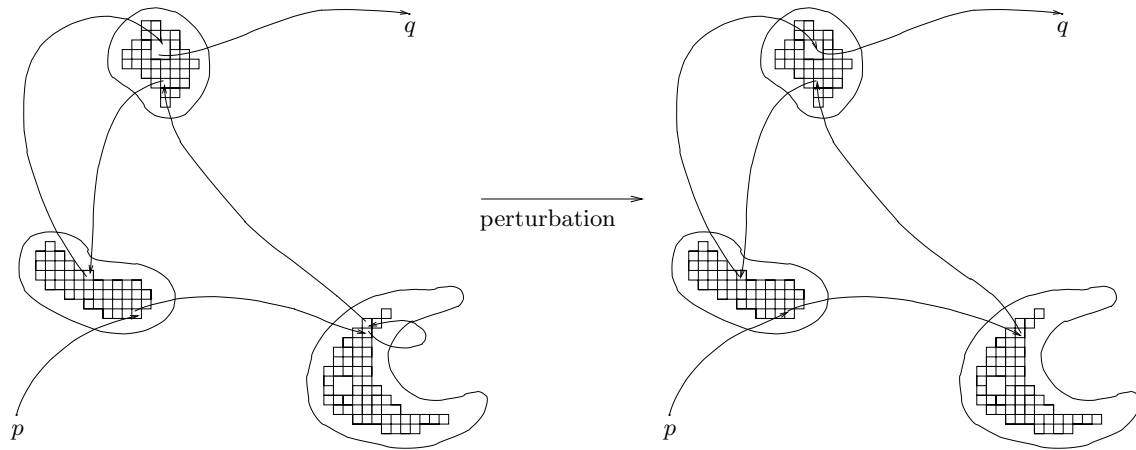
Figure 22: Final perturbation.
