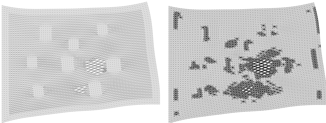
Figure 11: Solution obtained using the arc-length procedure after the limit point (left). On the right, the black bars are connected to the nodes corresponding to the highest values of the residual of the complete nonlinear system. They are mainly located in the zone of high topological changes.
