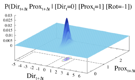
Figure 3: Example of probability distribution learned for the prediction term P(Dir_{t+\Delta} Prox_{t+\Delta} | Dir_t Prox_t Rot BM_{prox}) , with \Delta t = 900 ms. The prediction term for the starting location Dir_t = 0 , Prox_t = 1 and motor command Rot = -1 . The plot shows that if the robot had the wall in front of it, at a medium distance, and it turned to the left ( Rot = -1 ), then the wall would probably be on the right front side of the robot 900 ms later.
