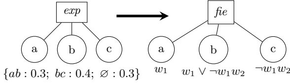
Figure 4: Translation from \text{PrXML}^{\text{exp}} to \text{PrXML}^{\text{fie}} , where p(w_1) = 0.3 ; p(w_2) = 0.4/0.7
