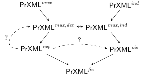
Figure 3: Efficient translations between \text{PrXML} families
