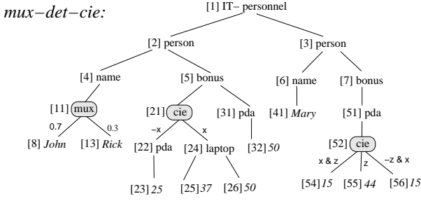
Figure 2: \text{PrXML}^{mux, det, cie} p-document: IT dpt.
