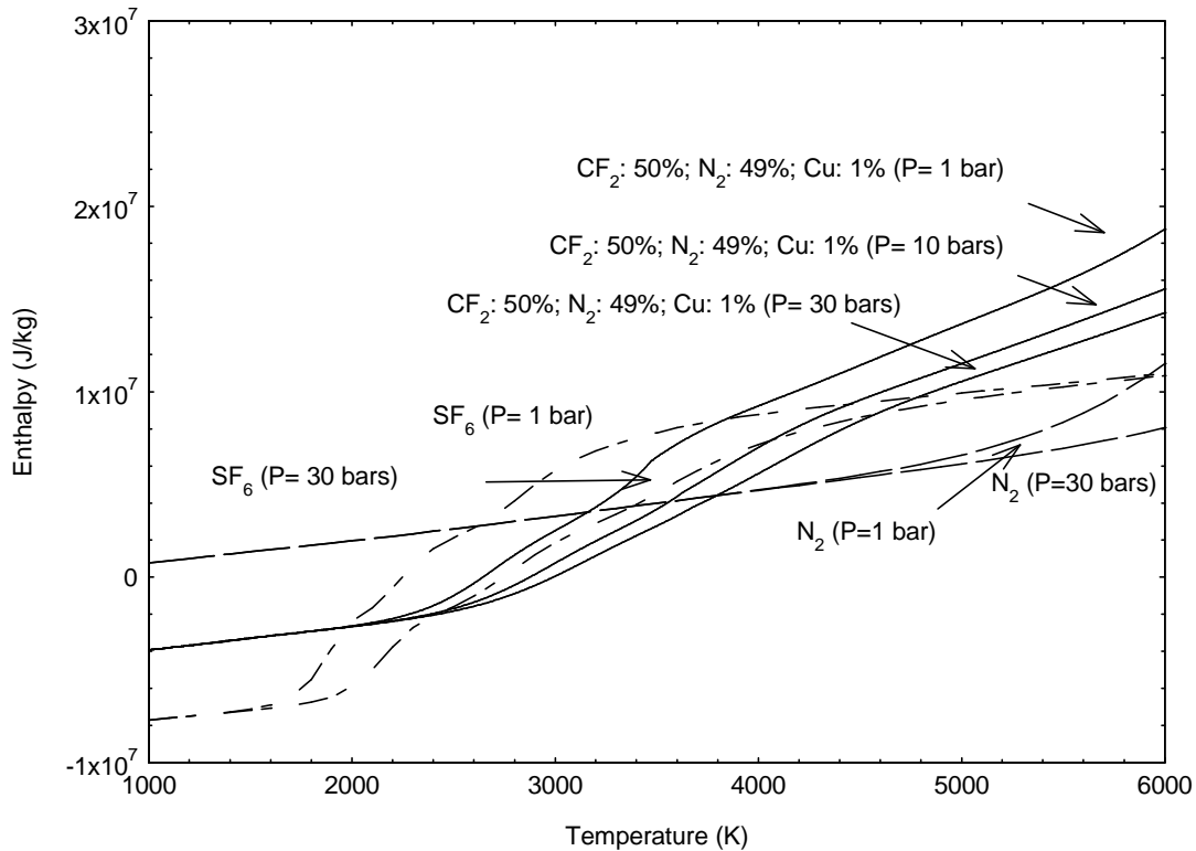
Figure 3.b: Massic enthalpy versus temperature for case 2, SF 6 and N 2 at tree pressures (1, 10 and 30 bars)
