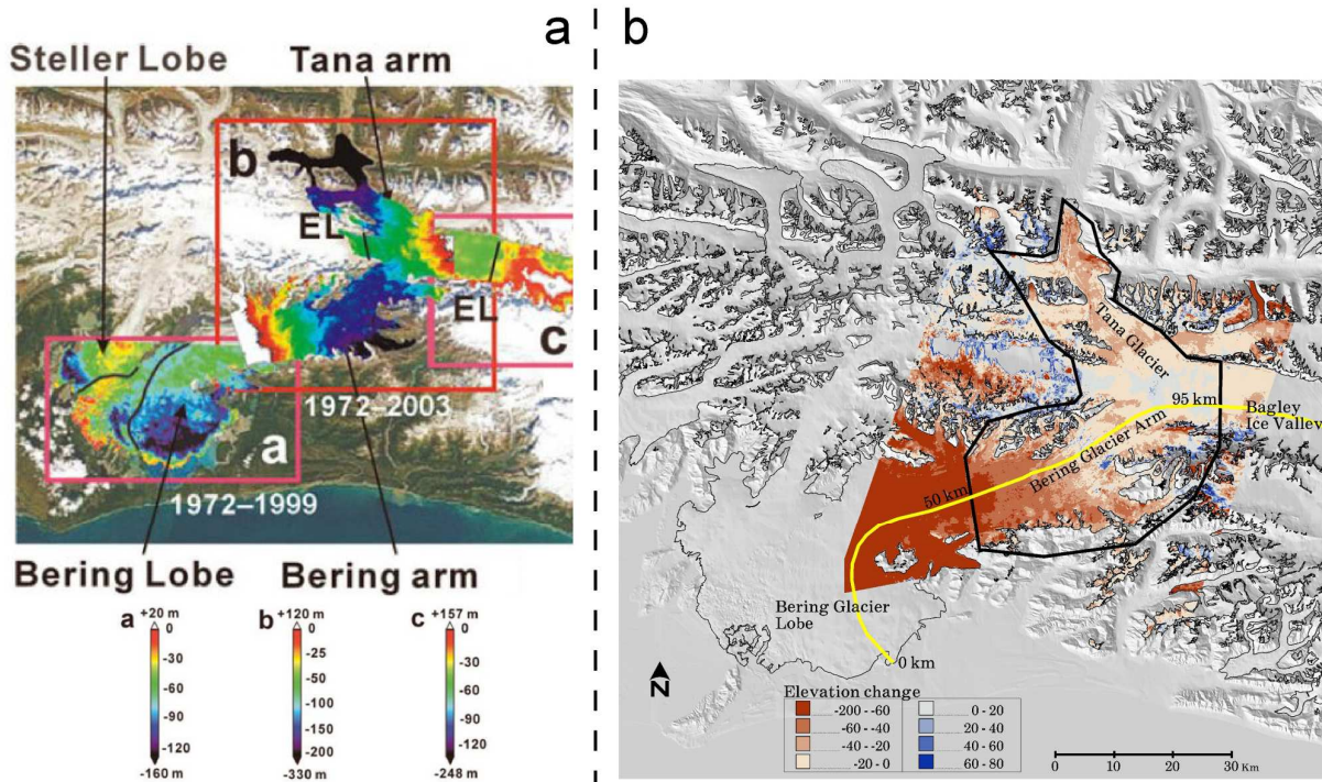
Figure 1: Elevation changes on the lower parts of Bering and Tana glaciers between 1972 and 2003; (a) reproduced from Figure 5 in M09 (see their legends for details); (b) calculated in this study. In the right panel, the background image is a shaded relief USGS DEM. The thin black line delimits the ice-covered areas extracted from the 1972 USGS maps (Berthier and others, 2010). The thick black polygon limits the area where volume change was derived by M09 using the ASTER-derived 2003 DEM. The yellow line locates the laser altimetry profile that was used by M09 in their Figure 6a. Distances along the laser altimetry profile are indicated.
