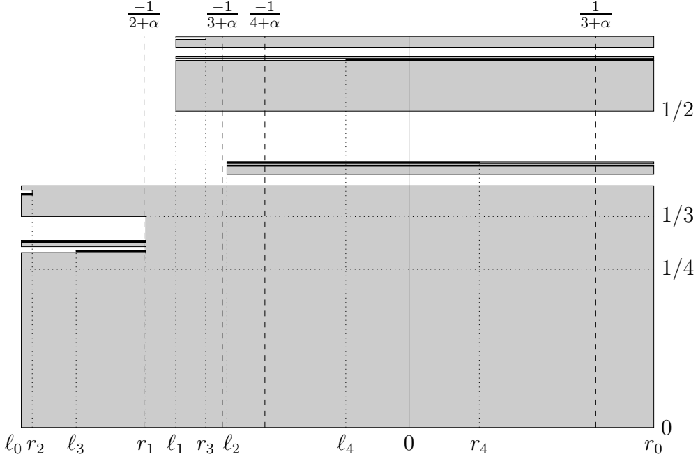
FIGURE 7. The domain \Omega_\alpha for \alpha = 113/292 \in \Gamma_{(-1:2)(-1:3)(-1:4)(-1:2)} , with l_j = T_\alpha^j(\alpha - 1) and r_j = T_\alpha^j(\alpha) .
