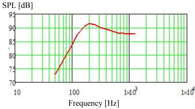
Fig. 2. Frequency response of the loudspeaker with inductance and eddy current resistor but without nonlinearity
