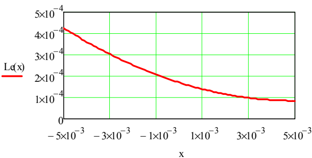
Fig. 15. The dependence of voice-coil inductance on displacement
