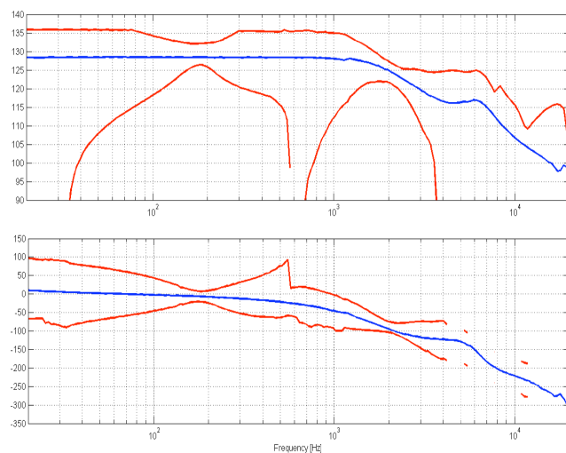
Figures 1 : Typical Frequency Response Bounds for a Loudspeaker, including Gain (upper) and Phase (lower), Nominal (blue) and Limits (red)
