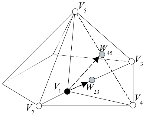
Fig. 13. Geometrical criterion for mesh simplification: V_1 is a sharp vertex and cannot be removed properly if it has V_4 and V_5 as parent vertices. On the other hand, it can be removed if its parent vertices are V_2 and V_3 , since this removal won't change the geometry significantly.
