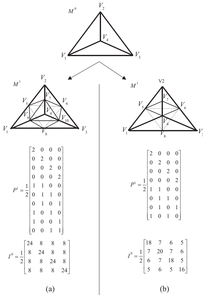
Fig. 15. Regular vs irregular subdivision of a tetrahedron : (a) regular case where all the faces are quadrisectioned. (b) irregular case where a face is split into four faces, two faces are split into three faces and one face is split in two
