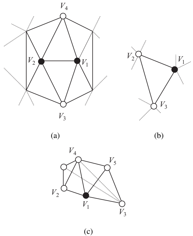
Fig. 10. Forbidden simplification cases: (a) two vertices V_1 and V_2 have the same parent vertices V_3 and V_4 ; (b) the vertex V_1 has V_2 and V_3 as parent vertices, but the edge V_1V_2 exists; (c) the edge flip that would change V_1V_5 to V_3V_4 is not allowed as V_3V_4 already exists in the mesh. On the other hand, flipping V_1V_4 to V_2V_5 is allowed
