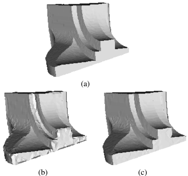
Fig. 14. Approximations of the "fandisk" mesh: (a) original mesh (6475 vertices), (b) mesh simplification without geometry criterion (2266 vertices) : some sharp edges were removed, (c) mesh simplification with a geometric criterion (2438 vertices): sharp edges are well preserved, keeping the visual aspect of the approximation close to the original mesh.
