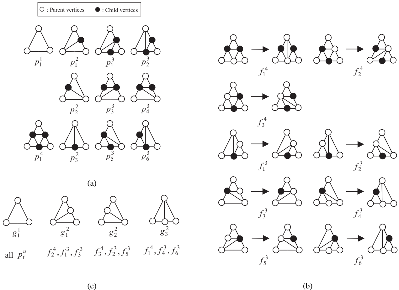
Fig. 9. Codebooks : (a) Wavelet Codebook W = \{p_i^u\} ; (b) Incident Codebook I = \{f_e^u\} ; (c) Merge Codebook M = \{g_i^u\}
