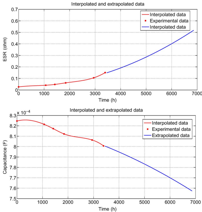
Fig. 13. ESR evolution at 5 kHz and C evolution at 200 Hz for one capacitor ( 1000 \mu\text{F}/450 \text{ V} ).
