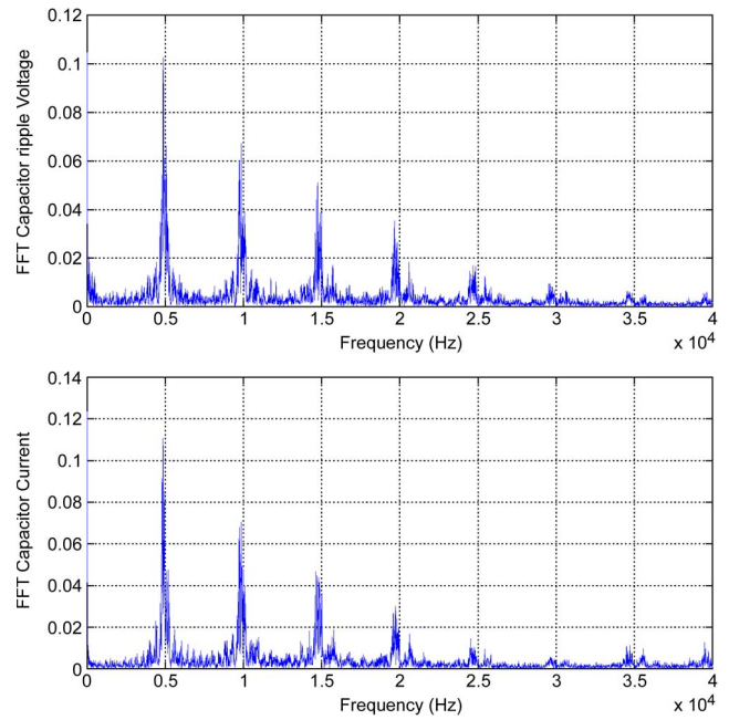
Fig. 14. FFT analysis of capacitor ripple voltage and capacitor voltage for a sampling frequency f_s = 80 \text{ kHz} .
