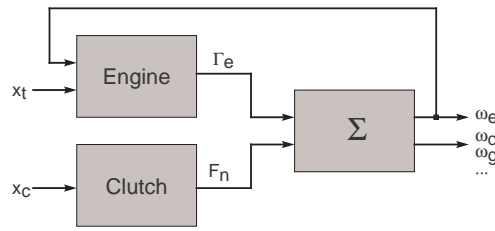
Fig. 2.8. Interconnection scheme of the model's three parts
