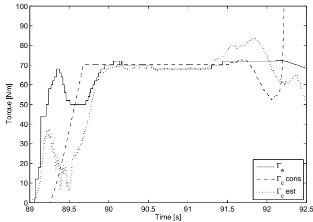
Fig. 7.14. Engine torque, requested clutch torque and estimated clutch torque relative to the standing start operation in Figure 7.12
