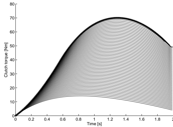
Fig. 5.5. Standing start simulation for a Clio II 1.5dCi (K9K) with a saturated ramp engine torque profile. The stars mark the optimization starting point for the optimal clutch torque trajectories drawn as a solid line.
