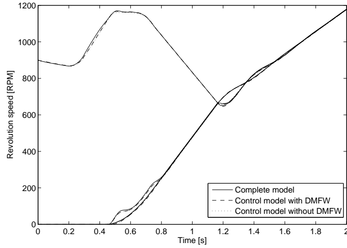
Fig. 2.14. Standing start simulations on flat ground using the same pedal position profiles and a complete driveline model, a simplified model including a liberalized DMFW and a simplified model without DMFW. Models parameters represent a 2.0l gasoline (F4R) Megane II.
