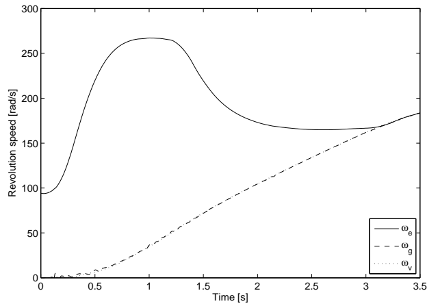
Fig. 5.11. Engine, gearbox and equivalent vehicle speed simulation results for a standing start simulation with a 10 segment MPC strategy; after 1.2 seconds of engagement the throttle position is reduced from 20% to half of its value
