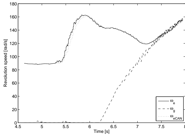
Fig. 7.15. Capture of a standing start on flat ground of the Clio II AMT prototype showcasing the suboptimal synchronization assistance strategy
