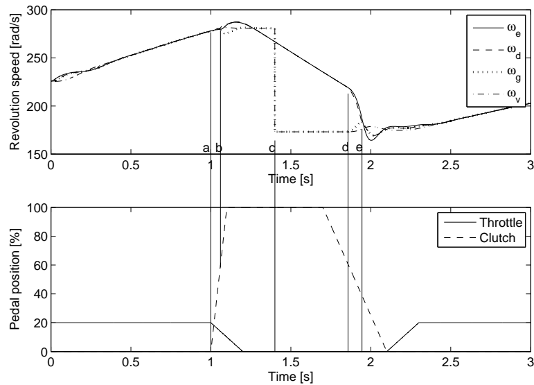
Fig. 3.2. Simulation of a throttle-less 1-2 upward gearshift. a beginning of the gearshift - b clutch disengagement - c new gear engagement - d beginning of the slipping phase - e synchronization.
