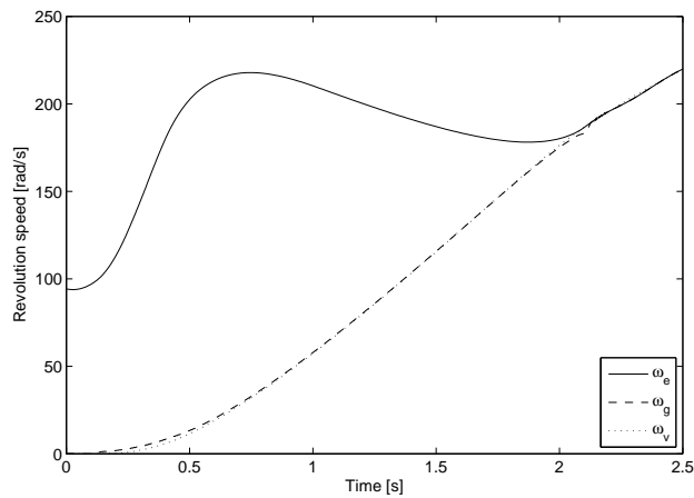
Fig. 5.6. Standing start simulation using the MPC strategy on a Clio II 1.5dCi (K9K) with a complete driveline with a torque generation model and a controlling driver model. A comfortable engagement is assured in spite of the strong changes in the engine torque.
