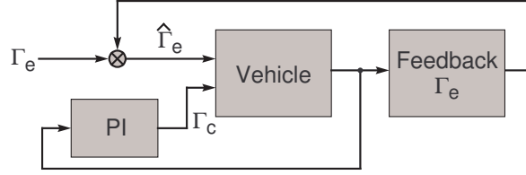
Fig. 4.5. Structure of the PI control with a sliding speed feedback and pole placement through engine torque control to increase the damping coefficient
