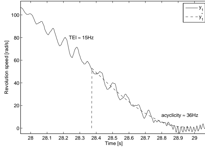
Fig. 7.7. Example of trajectory tracking, the measured sliding speed is drawn as a solid line while the optimal trajectory is dashed. A TEI oscillation is visible before the synchronization while after it the higher frequency engine acyclicity is present.
