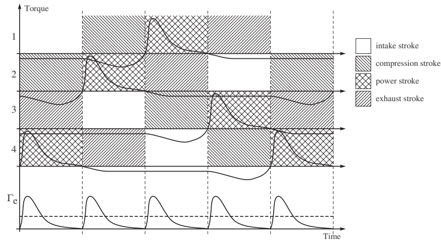
Fig. 2.4. Schematic representation of the output torque for each piston in a four cylinder engine having a standard 1342 ignition pattern. The last line shows the total instantaneous output torque and its \Gamma_e mean value over an half revolution.
