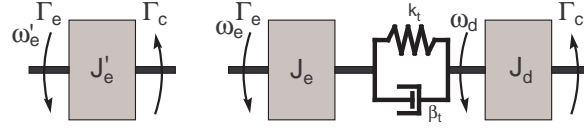
Fig. 6.3. Model of the driveline part upstream of the clutch
