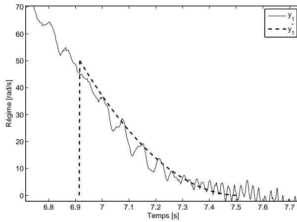
Fig. 7.16. Clutch sliding speed relative to the standing start operation shown in Figure 7.15. Due to the linear decrease of the clutch torque the suboptimal reference trajectory is simply an arc of a parabola.
