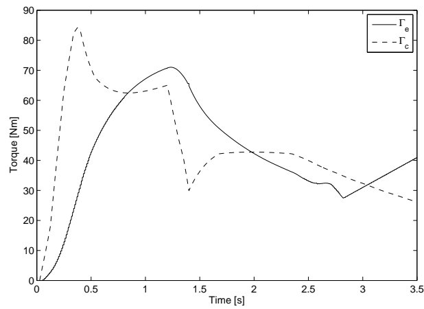
Fig. 5.12. Engine and clutch torque simulation results for a standing start simulation with a 10 segment MPC strategy; after 1.2 seconds of engagement the throttle position is reduced from 20% to half of its value
