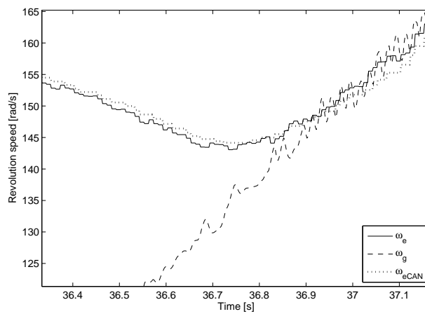
Fig. 7.9. Detail of Figure 7.8 highlighting the effect of the clutch partial reopening
