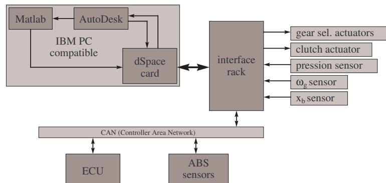
Fig. 7.4. Simplified connection diagram of the dSpace ® system
