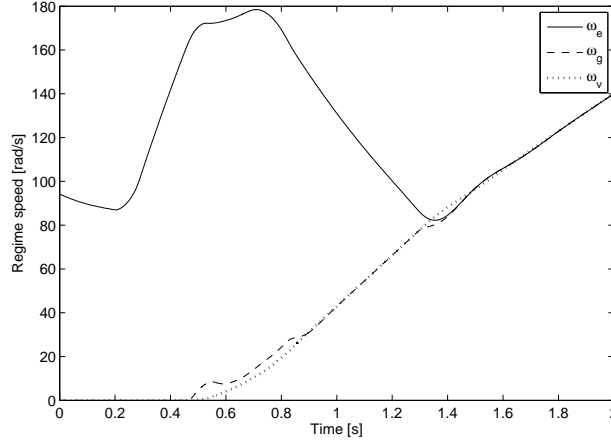
Fig. 4.4. Standing start simulation on flat ground with a synchronization assistance strategy based on a simple proportional feedback law. A 5% error on the friction coefficient \gamma causes a failed synchronization.
