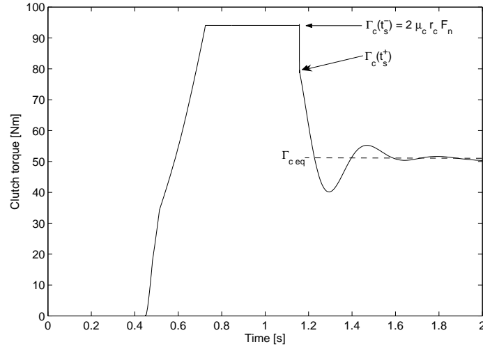
Fig. 3.4. Clutch torque during a simulated standing start
