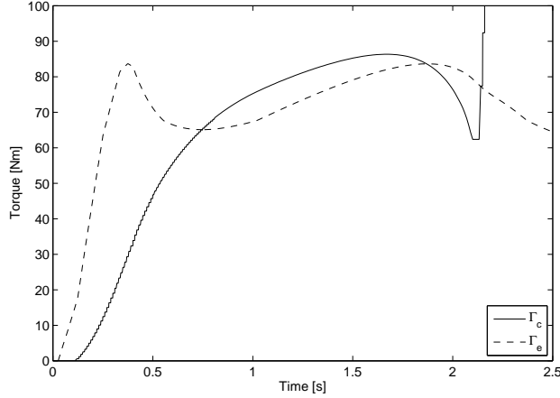
Fig. 5.7. Standing start simulation using the MPC strategy on a Clio II 1.5dCi (K9K) with a complete driveline with a torque generation model and a controlling driver model. A comfortable engagement is assured in spite of the strong changes in the engine torque.
