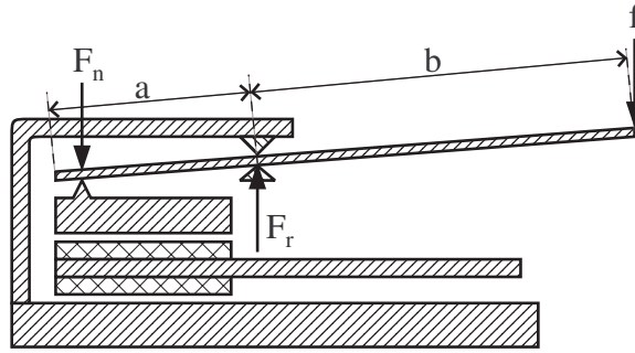
Fig. 2.6. Forces acting on the washer spring
