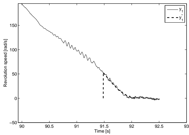
Fig. 7.13. Clutch sliding speed relative to the standing start operation shown in Figure 7.12. Due to the ballast load the derivative of the sliding speed is noticeably lower than the forecasted one at the beginning of the optimal trajectory.
