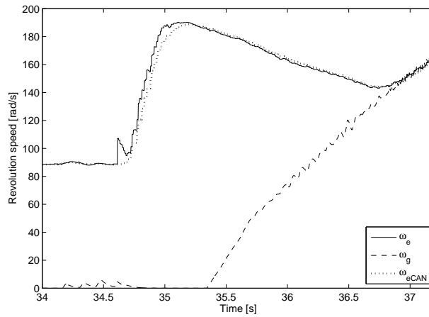
Fig. 7.8. Capture of a standing start on flat ground of the Clio II AMT prototype showcasing the synchronization assistance strategy. The optimal control is activated at 36.4 seconds and leads to a synchronization at 36.9 seconds slightly in advance over the optimal 37 seconds value.
