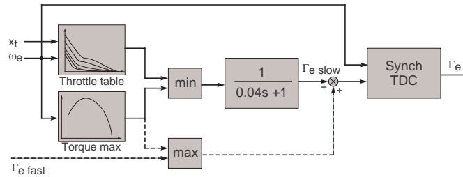
Fig. 2.9. Engine torque generation model for an indirect injection engine. The dotted part model an eventual torque reserve use. No filtering is present in case of a direct injection engine.
