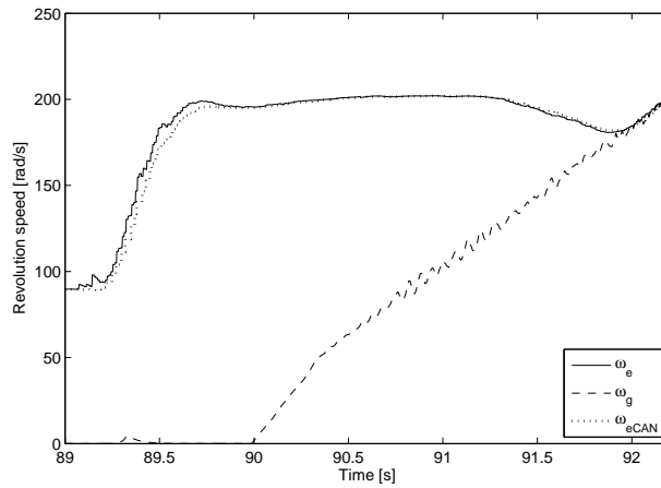
Fig. 7.12. Capture of a standing start on flat ground of the Clio II AMT prototype showcasing the synchronization assistance strategy robustness under a 400kg ballast load
