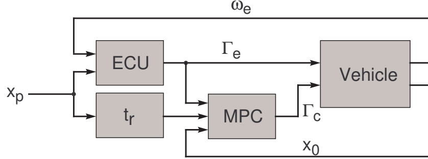
Fig. 5.2. Control structure of a MPC engagement control strategy for a AMT vehicle. The throttle pedal position x_p is the only system input, the engine control unit ECU outputs the engine torque target \Gamma_e based on x_p and \omega'_e . The control horizon is function of x_p and the clutch torque is controlled by the MPC strategy based on the driveline state x_0 , the control horizon length t_r and the engine torque.
