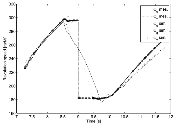
Fig. 2.12. Driveline model validation for a 1-2 gearshift on a Megane II equipped with a 2.0 gasoline engine (F4R)
