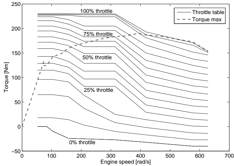
Fig. 2.3. Throttle look-up table for a gasoline engine traced in solid black together with the maximum output torque for a given engine speed traced in dashed grey
