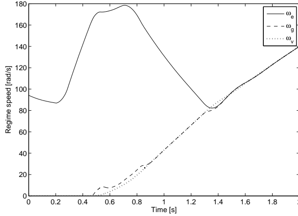
Fig. 4.3. Standing start simulation on flat ground with a synchronization assistance strategy based on a simple proportional feedback law
