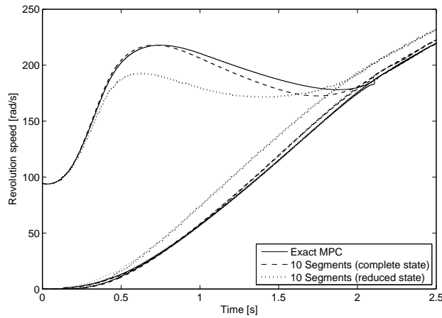
Fig. 5.9. Engine, gearbox and vehicle equivalent speeds for a standing start simulation of a Clio II on flat ground using the exact, segment approximated and reduced state segment approximated MPC strategy
