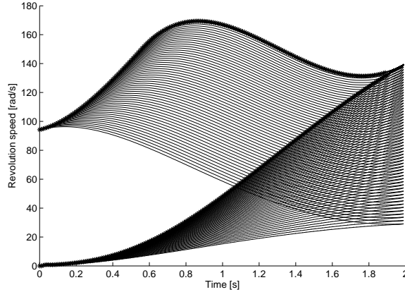
Fig. 5.4. Standing start simulation for a Clio II 1.5dCi (K9K) with a saturated ramp engine torque profile. The stars mark the optimization starting point.
