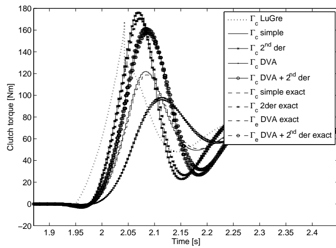
Fig. 6.6. Results of the clutch torque observers for a simulated fast 1-2 upshift with a sliding time of just 0.05 seconds
