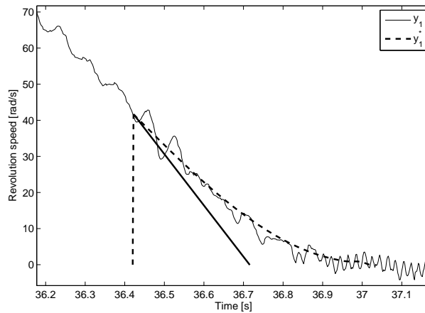
Fig. 7.10. Clutch sliding speed relative to the standing start operation shown in Figure 7.8. The thin solid line is the measured trajectory, the dashed line is the optimal reference trajectory and the black bold straight line shows the profile the sliding speed would have followed if no synchronization assistance was present.
