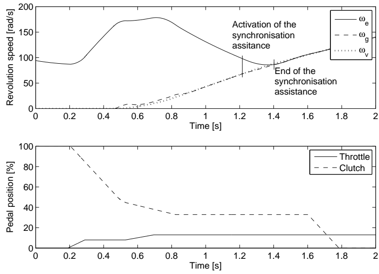
Fig. 4.1. Standing start simulation with a synchronization assistance strategy
