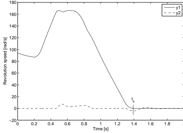
Fig. 4.7. Plot of the y_1 and y_2 speed differences for a standing start simulation with a synchronization assistance strategy based on a simple proportional feedback. Although the GV no-lurch condition is met at t_s , y_2(t_s) \neq 0 causes some residual oscillations.
