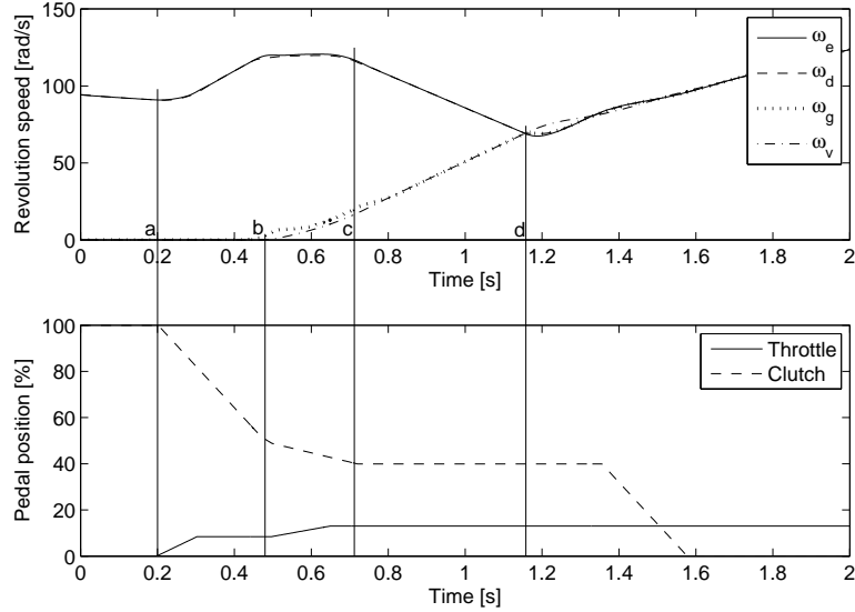
Fig. 3.1. Simulation of a standing start on flat ground. a beginning of the standing start - b contact point - c desired acceleration level is reached - d synchronization.
