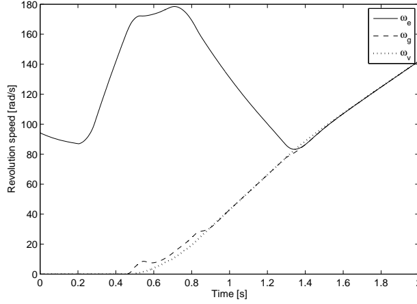
Fig. 4.6. Standing start simulation on flat ground with a synchronization assistance strategy based on a PI controller with an additional feedback loop on the engine torque
