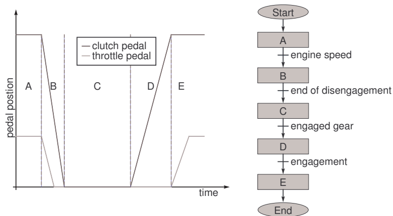
Fig. 2.16. Finite state machine generating the throttle and clutch pedal positions for a gearshift.
