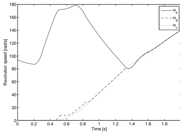
Fig. 4.2. Simulation of a standard standing start for an MT vehicle on flat ground
