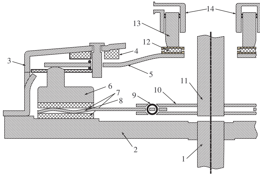
Fig. 2.5. Clutch structure, axial cut. 1 crankshaft - 2 flywheel - 3 clutch external structure - 4 wear compensation system - 5 washer spring - 6 pressure plate - 7 friction pads - 8 flat spring - 9 spring damper - 10 clutch disk - 11 gearbox primary shaft - 12 needle roller bearing - 13 Concentric Slave Cylinder (CSC) piston - 14 Concentric Slave Cylinder (CSC)
