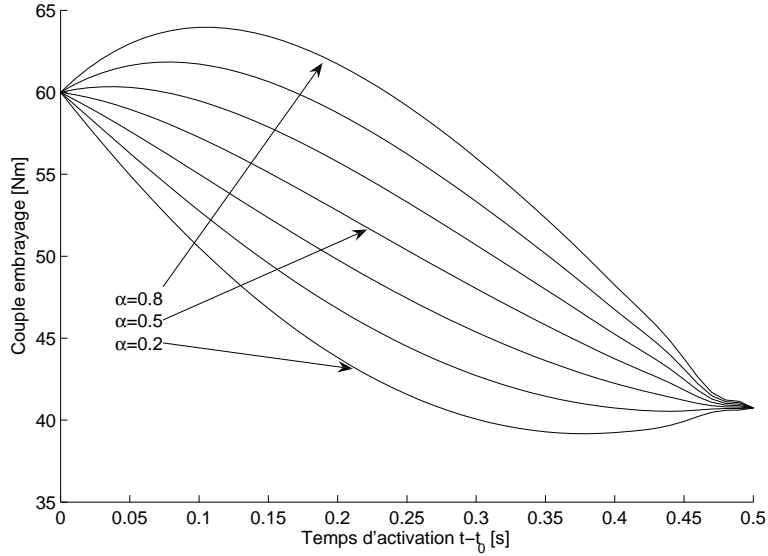
Fig. 4.11. Clutch torque optimal engagement trajectories for a Clio II over an activation interval of t_s - t_0 = 0.5 seconds, \Gamma_e(t_0) = 50Nm , \Gamma_c(t_0) = 60Nm and \alpha \in [0.2, 0.8]
