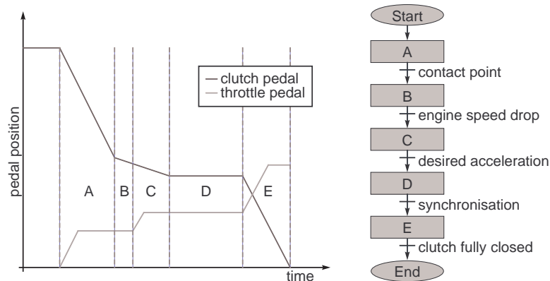
Fig. 2.15. Finite state machine generating the throttle and clutch pedal positions for a standing start.
