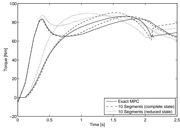
Fig. 5.10. Engine and clutch torques for a standing start simulation of a Clio II on flat ground using the exact, segment approximated and reduced state segment approximated MPC strategy
