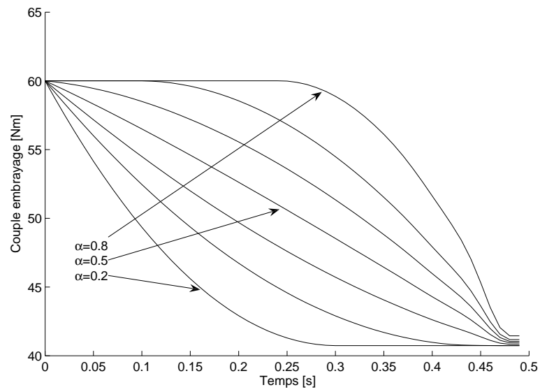
Fig. 4.12. Clutch torque optimal engagement trajectories for a Clio II over an activation interval of t_s - t_0 = 0.5s , \Gamma_e(t_0) = 50Nm , \Gamma_c(t_0) = 60Nm and \alpha \in [0.2, 0.8] and subject to the inequality constraints u \leq 0 and y_1 \geq 0
