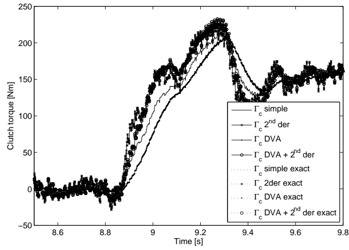
Fig. 6.5. Results of the clutch torque observers for a 1-2 upshift using actual data measured on a Megane II 2.0 essence (F4R)
