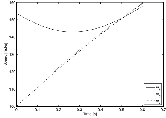
Fig. 4.8. Optimal synchronization trajectories obtained through an LQ formulation with a = 1 , b = 10^{-2} and \epsilon = 10^{10}
