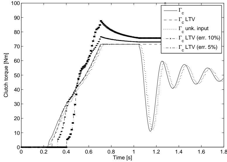
Fig. 6.2. Results of the clutch torque estimation \Gamma_c for a simulated standing start on flat ground for a Clio II 1.5dCi (K9K) using the unknown input observer and the MIMO-LTV with \Gamma_c = \hat{\gamma}F_n for the nominal case and for a 5% and 10% error on the contact point
