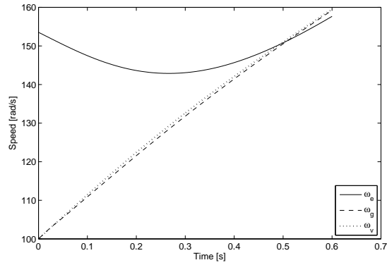
Fig. 4.9. Optimal synchronization trajectories obtained through an LQ formulation with a = 1 , b = 10^{-2} and \epsilon = 10^{10}
