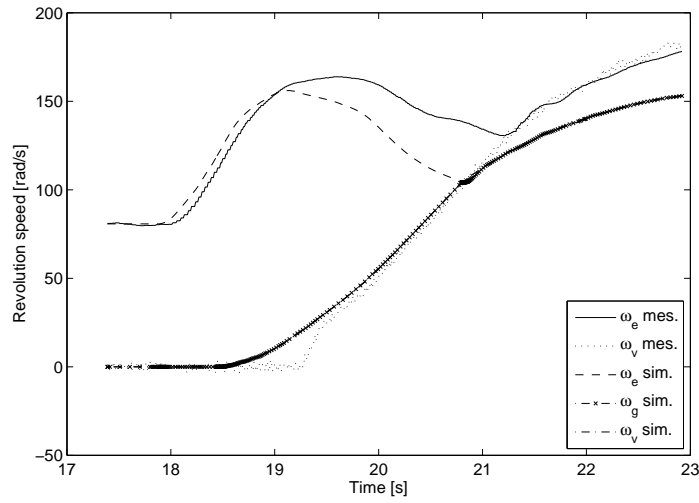
Fig. 2.11. Driveline model validation for a standing start of a Megane II equipped with a 2.0 gasoline engine (F4R)
