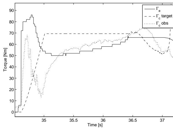
Fig. 7.11. Engine torque, requested clutch torque and estimated clutch torque relative to the standing start operation in Figure 7.8. The clutch partial reopening reduces the transmitted torque from its initial value of almost 70Nm to about 50Nm with an engine torque of 66Nm .
