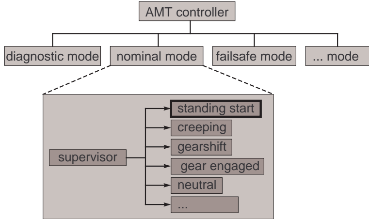
Fig. 7.5. Idealized representation of the AMT gearbox controller internal structure. When in nominal mode the supervisor manages the activation of the various modules.
