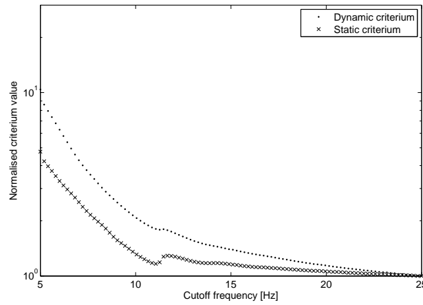
Fig. 3.5. Evolution of the static and dynamic criteria for the low pass filtering action as a function of the cutoff frequency. Results have been normalized with respect to the results obtained for a 25\text{Hz} cutoff frequency.
