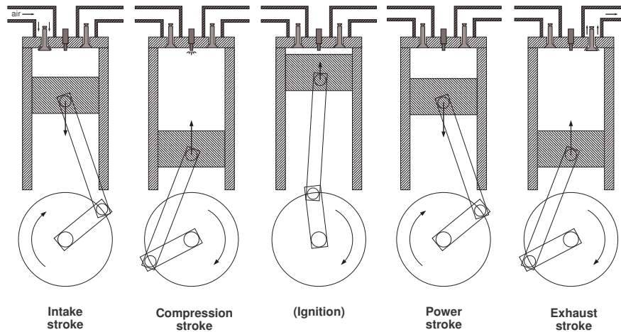
Fig. 2.2. Diesel engine four-stroke cycle
