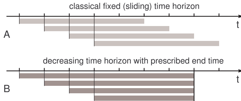
Fig. 5.1. Optimization horizon update for a sliding horizon (A) and a fixed horizon (B) formulations
