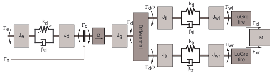
Fig. 2.10. Advanced simulation model with 14 degrees of freedom
