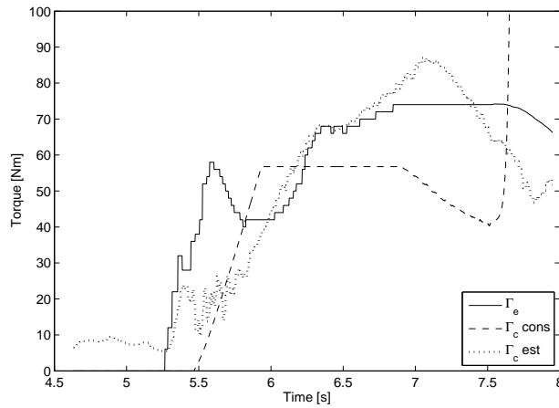
Fig. 7.17. Engine torque, requested clutch torque and estimated clutch torque relative to the standing start operation in Figure 7.15. The linear decrease of torque is clearly visible at the end of the engagement. It can also be noted that, due to a change of the clutch characteristic, while the target value of \Gamma_c is lower than \Gamma_e , the value estimated by the unknown input observer is higher than the engine torque which is consistent with the decrease of engine speed shown in Figure 7.15.
