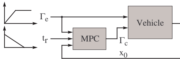
Fig. 5.3. Structure of the simplified case used to validate the principle of the fixed horizon MPC strategy
