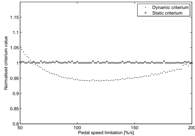
Fig. 3.6. Evolution of the static and dynamic criteria for the pedal speed limiter as a function of the speed limit. Results have been normalized with respect to the results obtained for a 200%/s limit speed.
