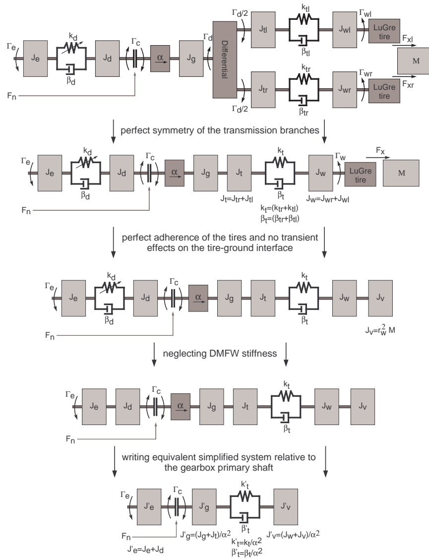
Fig. 2.13. Step-by-step derivation of the simplified model from the complete driveline model.
