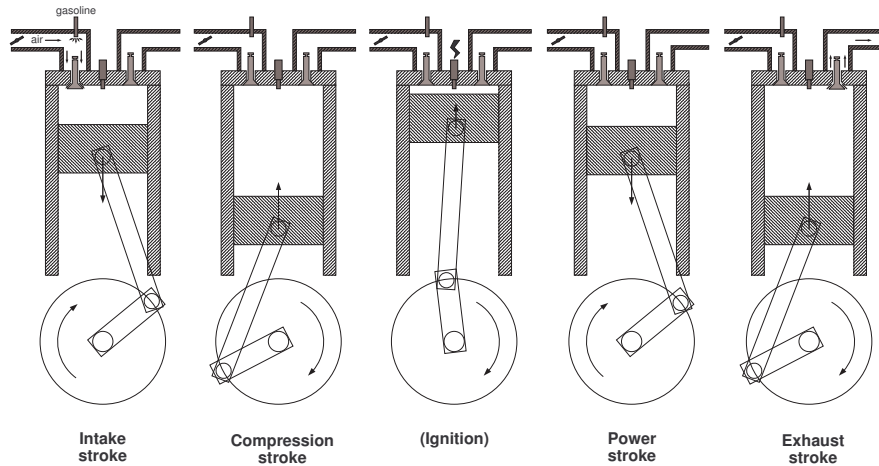
Fig. 2.1. Gasoline engine four-stroke cycle
