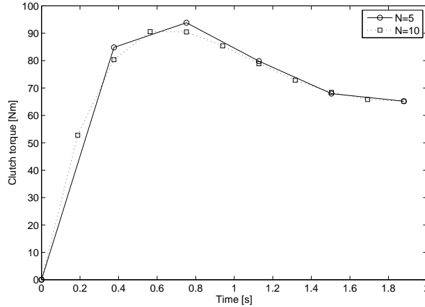
Fig. 5.8. Example of two optimal trajectories composed by 5 and 10 segments
