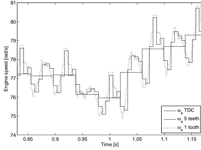
Fig. 6.4. Comparison between different engine speed measurements: the solid line is a standard twice-per-revolution measure over 30 teeth, the dashed line is a twelve-times-per-revolution measure over 5 teeth and the dotted line is a direct tooth-by-tooth measure obtained through an external 20KHz sampling
