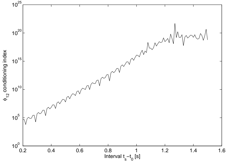
Fig. 4.10. Conditioning index of the \varphi_{12} matrix as a function of the length of the optimal control activation interval
