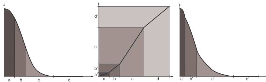
Fig. 3.7. Example of a variable reduction hydraulic control system; the high torque range has been reduced in favor of the initial part improving the dosability while assuring a contact point around 60% of the pedal stroke
