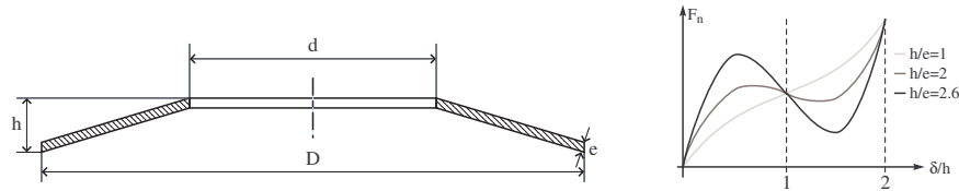
Fig. 2.7. Geometry of a washer spring and its stiffness curve for several values of h/e ratio
