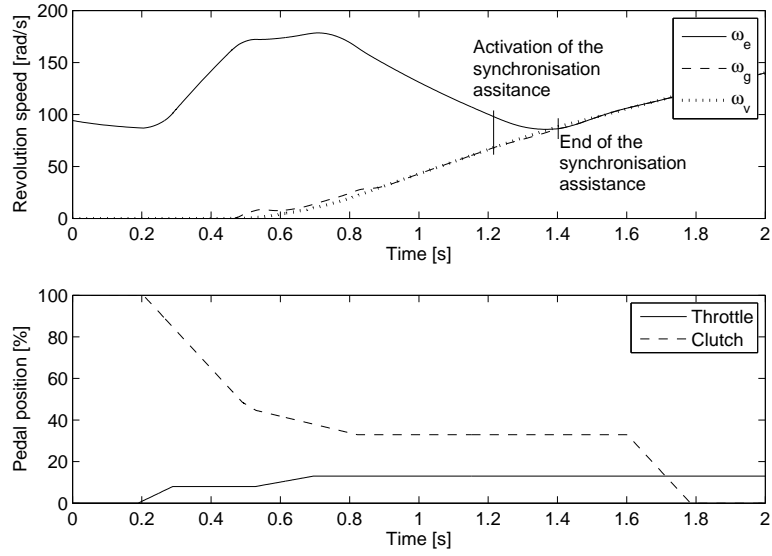
Fig. 4.1. Standing start simulation with a synchronization assistance strategy
