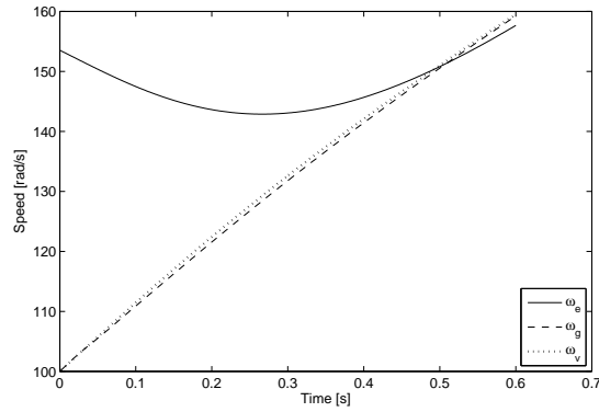
Fig. 4.9. Optimal synchronization trajectories obtained through an LQ formulation with a = 1 , b = 10^{-2} and \epsilon = 10^{10}
