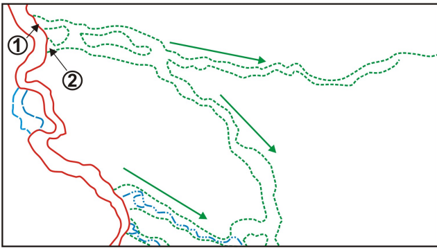
Figure 7: Satellite Image and interpretative map of the Great Diversion of the Pastaza are. Observe the sharp contrast between alluvial ridges (even abandoned and the floodplain area. 1) points of avulsion, 2) abandoned alluvial ridges, 3) abandoned loop of the Rio Pastaza, 4) underfitted streams re-occupying abandoned reaches, 5) modern Rio Pastaza Channel.
