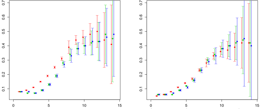
FIGURE 5. Confidence intervals of the estimates \hat{d}_{n,\text{CL}} (red), \hat{d}_{n,\text{CR}} (green) and \hat{d}_{n,\text{MAD}} (blue) on the data Thu1300 (left) and Sat1930 (right) for J_0 = 1, \dots, 14 and J_0 + \ell = 19 .
