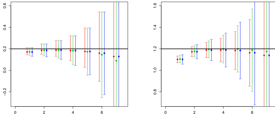
FIGURE 1. Confidence intervals of the estimates \hat{d}_{n,CL} , \hat{d}_{n,CR} and \hat{d}_{n,MAD} of an ARFIMA(0, d , 0) process with d = 0.2 (left) and d = 1.2 (right) for J_0 = 1, \dots, 8 and J_0 + \ell = 9 . For each J_0 , are displayed confidence interval associated to \hat{d}_{n,CL} (red), \hat{d}_{n,CR} (green) and \hat{d}_{n,MAD} (blue), respectively.
