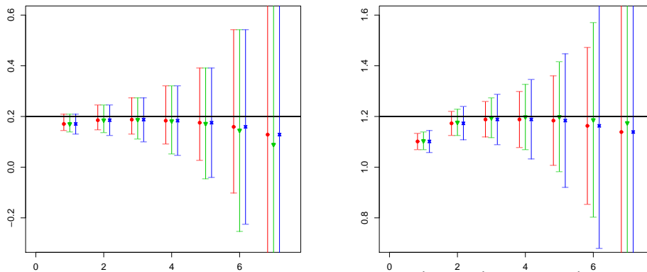
FIGURE 1. Confidence intervals of the estimates \hat{d}_{n,\text{CL}} , \hat{d}_{n,\text{CR}} and \hat{d}_{n,\text{MAD}} of an ARFIMA(0, d ,0) process with d = 0.2 (left) and d = 1.2 (right) for J_0 = 1, \dots, 8 and J_0 + \ell = 9 . For each J_0 , are displayed confidence interval associated to \hat{d}_{n,\text{CL}} (red), interval \hat{d}_{n,\text{CR}} (green) and \hat{d}_{n,\text{MAD}} (blue), respectively.
