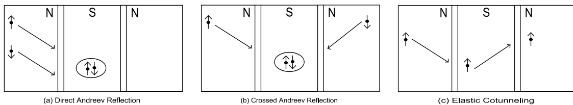
FIG. 4: Dominant electron transfer processes
