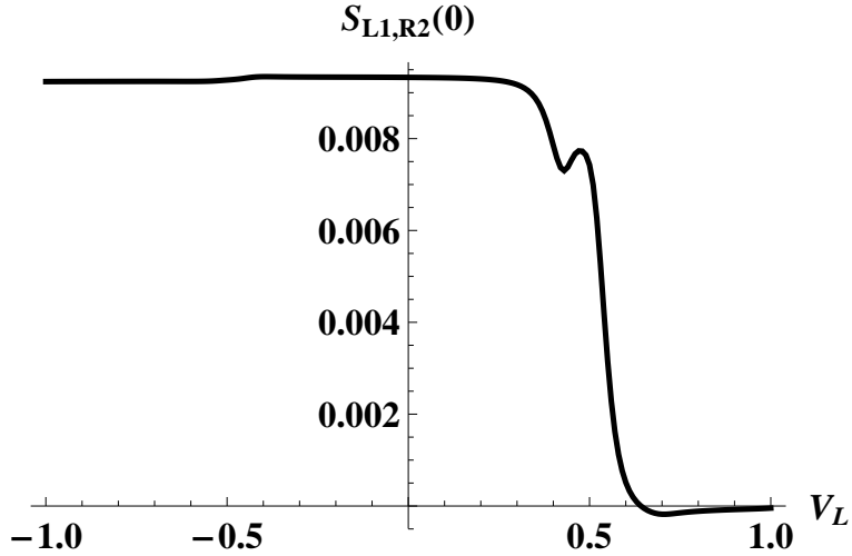
FIG. 8: Current-current crossed correlation S_{L1,R2}(0) (between I_{L1} and I_{R2} ) at zero frequency (arbitrary units) as a function of the voltage of the left lead V_L for the same setup as in Fig. 6.
