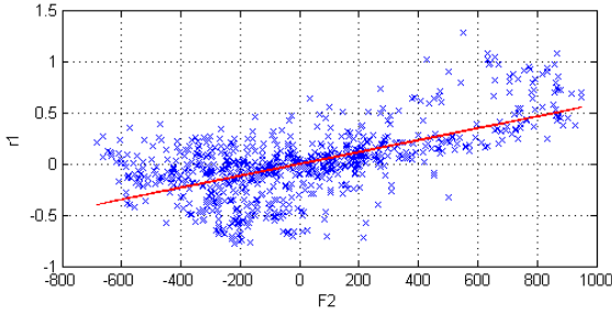
Figure 3: r_1 values (crosses) and its estimation (straight line) in function of F_2 .
