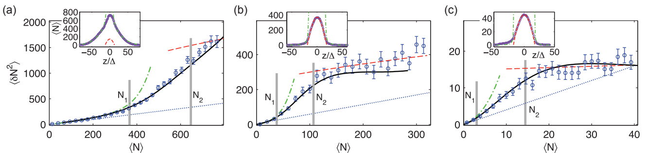
FIG. 1. Density fluctuations across the quasi-condensate transition, for k_B T / \hbar \omega_\perp = 3.6 (a), 1.0 (b) and 0.09 (c). The measured atom-number variances in individual pixels, \langle \delta N^2 \rangle , as a function of the mean atom number \langle N \rangle are shown as circles, with the error bars representing the statistical uncertainty. Different curves are the predictions from theoretical models, rescaled by the resolution factor \kappa = 0.53, 0.55 and 0.4 for (a), (b) and (c), respectively (see text): modified Yang-Yang model (solid), ideal Bose gas (dash-dotted), quasi-condensate (dashed) and the Poissonian shot-noise level (dotted). The two vertical gray lines give the atom numbers N_1 = \Delta n_1 and N_2 = \Delta n_2 (see text). The insets show the average density profiles, together with the predictions from the same models (different curves are as in the main graphs). The chemical potential \mu_0 in the trap center is deduced from the fit of the wings of the density profile to the ideal Bose gas EoS for (a), and from the peak density and the quasi-condensate EoS for (b) and (c). The trap oscillation frequencies are: \omega_\perp/2\pi = 3.0 kHz, \omega_\parallel/2\pi = 8.0(5) Hz for (a-b) and \omega_\perp/2\pi = 3.9 kHz, \omega_\parallel/2\pi = 4.0(5) Hz for (c). The absolute temperatures are T = 510 nK (a), 160 nK (b), and 18 nK (c).
