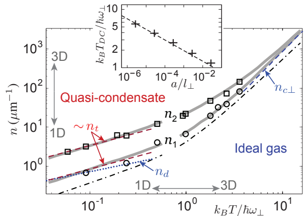
FIG. 2. Phase diagram in the 1D-3D crossover. The data at k_B T/\hbar\omega_{\perp} < 0.8 ( > 0.8 kHz) are taken with \omega_{\perp}/2\pi = 3.9 kHz ( = 3.0 kHz). The measured transition boundaries n_1 (circles) and n_2 (squares) are plotted along with the predictions from the MYYM (solid gray curves). The dash-dotted curve is the perturbative calculation of n_1 ; all other lines are as labeled (see text). The inset shows the dimensional crossover temperature T_{DC} versus a/l_{\perp} (crosses), fitted with a power law (a/l_{\perp})^{-2/11} (dashed line, see text).
