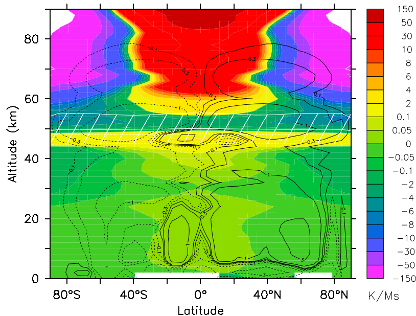
Figure 8. Radiative temperature tendency (sum of solar and infrared temperature tendencies), averaged over the last two days of the simulation (unit is 10^{-6} \text{ K s}^{-1} ). Contours show the temperature tendency due to convective adjustment (white, with the dominant convective region highlighted by the dashed area) and mass stream function (black, 10^9 \text{ kg s}^{-1} ).
