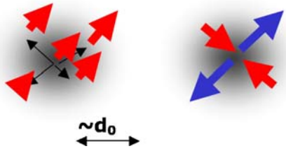
Fig. 11 Example of strain rate calculation. On the left figure five sites are present: one is at the center of a circle of radius equal to the typical correlation length of the ensemble of velocities, and four additional velocities are uniformly distributed about that point within the circle. On the right we have the corresponding strain rate eigenvectors. The structure of the velocity distribution is such that one expects an extension in the NE–SW direction. This deformation regime is then a mean property of the entire circular area
