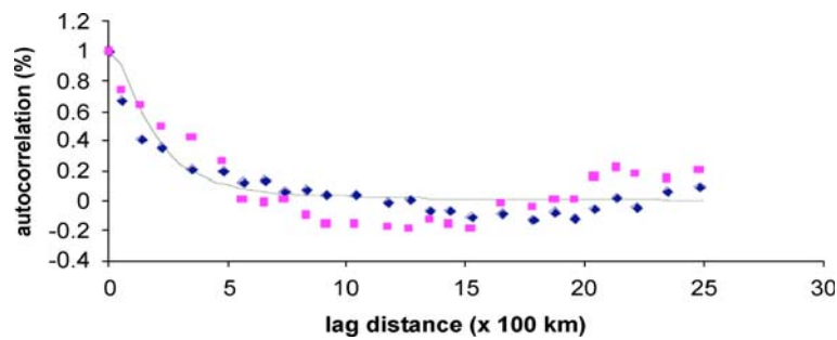
Fig. 10 The autocorrelation of the observed velocities as a function of the distance between stations. The continuous curve represents an analytical covariance function depend-
