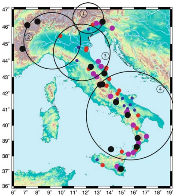
Fig. 3 M_0R (in N·m/year) computed by geophysical modelling for the seismogenic areas. Blue small dots for M_0R < 5.0 \times 10^{15} ; red medium dots 5.0 \times 10^{15} \leq M_0R < 1.0 \times 10^{16} ; purple medium circles 1.0 \times 10^{16} \leq M_0R < 3.0 \times 10^{16} ; black large circles M_0R \geq 3.0 \times 10^{16} . The numbered large circles identify the four domains: 1 eastern Alps, 2 western Alps, 3 central Apennines, 4 southern Apennines
