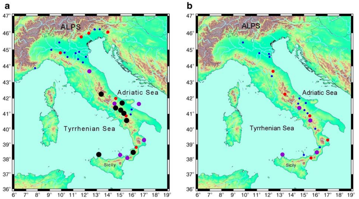
Fig. 7 Thirty-year probability for M_W \geq 6.5 according to a Poisson model: a computed by geodetic constraints, b computed by geophysical constraints. Blue small dots for
