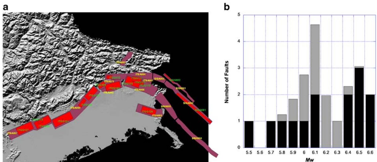
Fig. 5 Mapped and modelled faults in the eastern Alps domain: a seismogenic areas (purple areas marked by ITSA) and mapped faults (red areas marked by ITGG),
