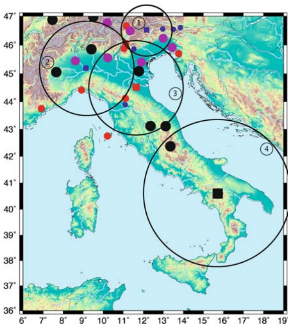
Fig. 2 M_0R (in N-m/year) computed from GPS observations. Blue small dots for M_0R < 1.0 \times 10^{18} ; red medium dots 1.0 \times 10^{18} \leq M_0R < 2.0 \times 10^{18} ; purple medium circles 2.0 \times 10^{18} \leq M_0R < 3.0 \times 10^{18} ; black large circles M_0R \geq 3.0 \times 10^{18} . The central GPS station of each domain is marked by a square with size and color according to its M_0R . The numbered large circles identify the four domains: 1 eastern Alps, 2 western Alps, 3 central Apennines, 4 southern Apennines
