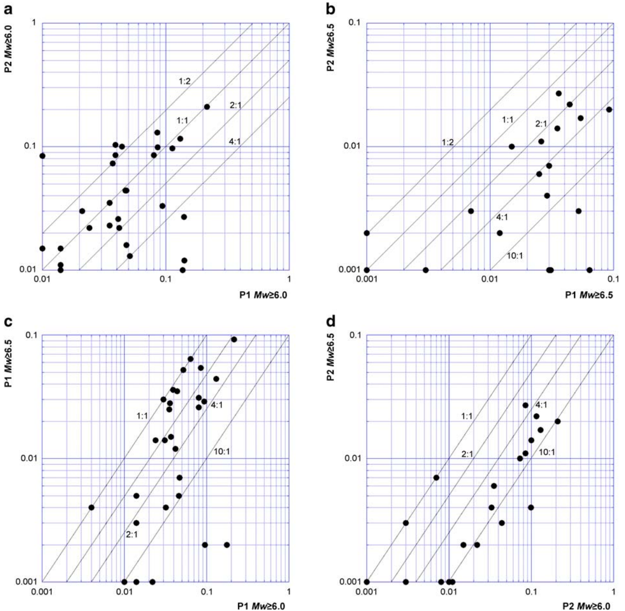
Fig. 8 Comparison of the probability estimates ( P1 indicates the exceedance probability in 30 years computed with geodetic constraints, P2 indicates the exceedance probability in 30 years computed with geophysical constraints):
