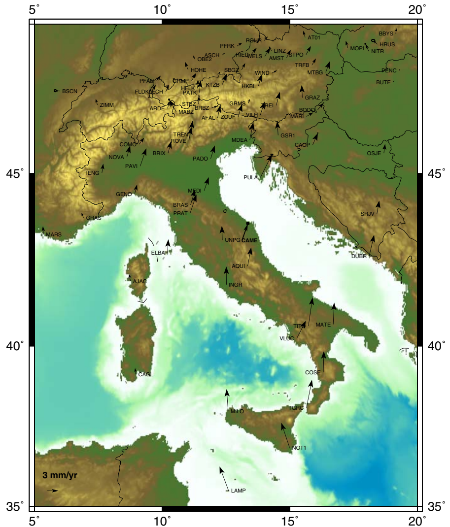
Fig. 9 Horizontal velocities of GPS permanent stations in the Alpine Mediterranean area, after removing a common rigid rotation which approximates the rigid rotation of the Eurasian plate in the ITRF2000 frame. Error ellipses are 2\sigma . Velocities have been computed only for stations with at least 2.5 years of continuous tracking. Not shown are the velocities of EPN stations falling outside the plotting box
