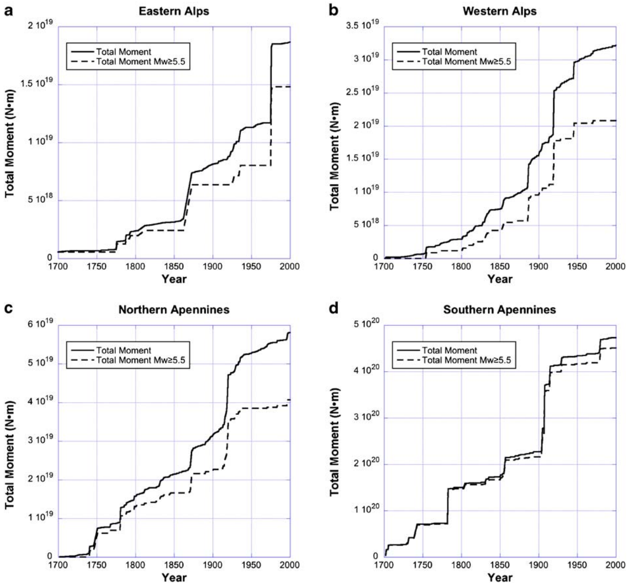
Fig. 4 M_0 release since 1700 in the four domains: a eastern Alps, b western Alps, c northern Apennines, d southern Apennines. Solid line for all earthquakes of the Italian
