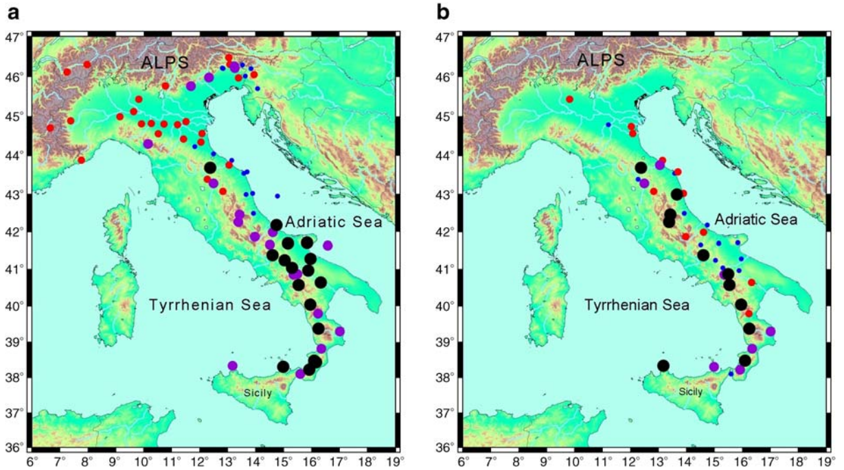
Fig. 6 Thirty-year probability for M_W \geq 6.0 according to a Poisson model: a computed by geodetic constraints, b computed by geophysical constraints. Blue small dots for
