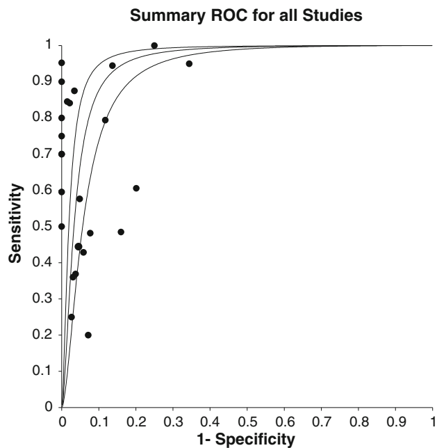
Fig. 1 The SROC for all studies included in the meta-analysis
