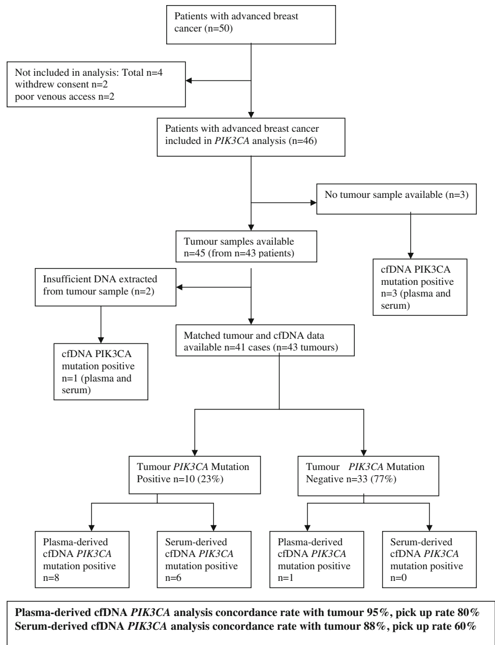
Fig. 1 Schema summarising PIK3CA mutation analysis on tumour and cfDNA in patients with advanced breast cancer
