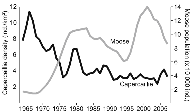
Fig. 1 The abundance estimates of capercaillie and moose, attained from wildlife triangle data, from 1964 to 2008
