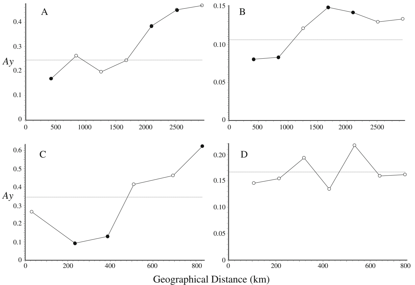
Fig. 4 Results of spatial autocorrelation analyses of raccoon dog sequences found in the the whole European dataset with (a) and without (b) clade II individuals, the drainage area of the Lake Päijänne in Finland (c) and the combined Oder and Elbe river basins in Germany (d). Analyses were performed using six to seven distinct distance classes. A_y quantifies the average pairwise genetic distances
