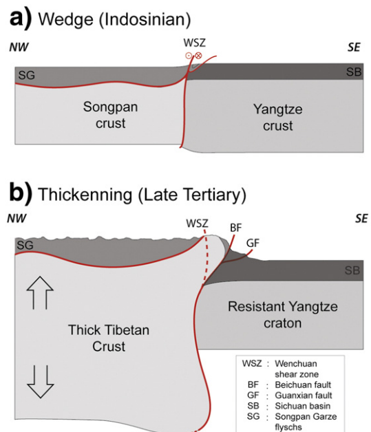
Fig. 7. Schematic scenario envisaged for the Longmen Shan along the geophysical profile. Top: During the early Indosinian event, the crust located west of the present Longmen Shan belonged to the margin of the Paleotethys and composed of a poorly known oceanic or thinned continental crust, and was adjacent to the continental crust of the Yangtze block. A detachment that separated the sedimentary units involved in a subduction wedge created sedimentary thickening and shortening (very oblique to the section). Bottom: Crustal thickening during the Neogene as a result from the India/Eurasia convergence overthrew material from the soft Tibetan crust and its upper part composed of the crystalline massifs onto the Yangtze block.
