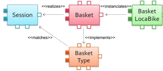
Fig. 5. BikeCourseDBClass composite component
