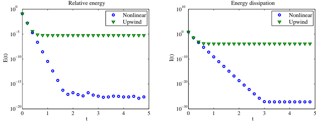
Figure 2: Nonlinear case: relative energy \mathcal{E}^n and dissipation \mathcal{I}^n for different schemes in log scale, with time step \Delta t = 5.10^{-4} and space step \Delta x = 10^{-2} .
