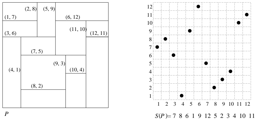
FIGURE 12. A floorplan P , with segments labeled (i, j) , where i (respectively, j ) is the label according to the \searrow (respectively, \swarrow ) order, and the corresponding S-permutation.
