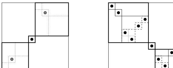
FIGURE 24. Separable-by-point permutations.
