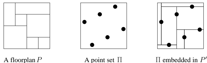
FIGURE 2. A rectangulation: embedding a point set \Pi in a floorplan P .
