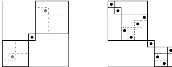
Figure 29: Separable-by-point permutations.
