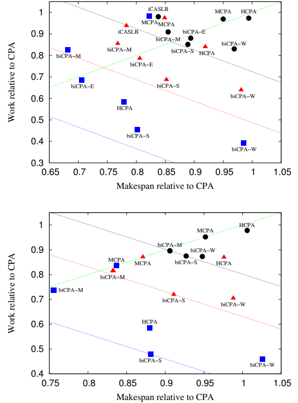
Figure 5. Bi-criteria average performance of all algorithms relatively to the CPA algorithm depending on the target cluster – small ( chti – ●), medium ( grillon – ▲) and large ( grelon – ■) – for PTGs without (top) and with (bottom) inter-task communications.
