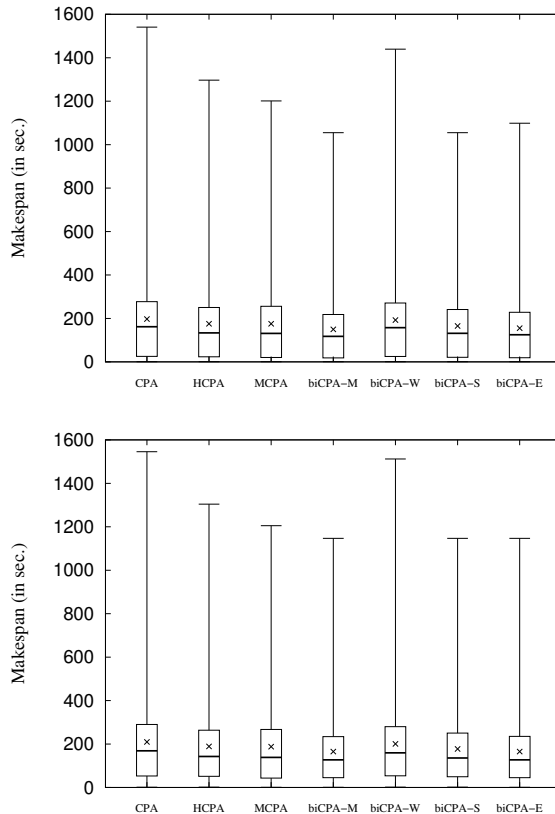
Figure 3. Distribution of overall makespan values for all algorithms for PTGs without (top) and with (bottom) inter-task communications.
