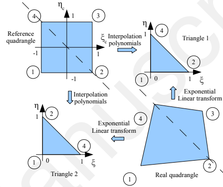
Figure 8 : FEA transformation of the linear quadrangle from real to reference coordinates via 2 pseudo-triangles
