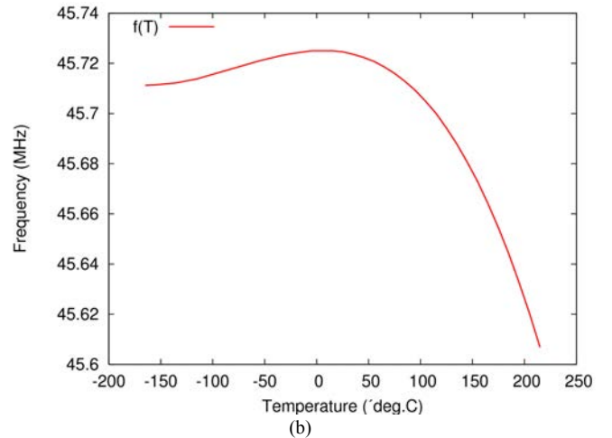
Figure 3. Thermal sensitivity of pure shear wave on (a) AT and (b) BT Quartz cuts computed along the proposed approach
