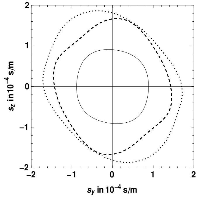
Figure 9 Slowness curves of r-plane sapphire used as substrate: a) XZ-plane b) YZ-plane. Solid line: fast shear wave, dashed line: slow shear wave, dotted line: longitudinal wave. Strong anisotropy of the material cause tilted Poynting vectors.
