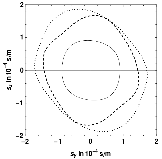
Figure 9 Slowness curves of r-plane sapphire used as substrate: a) XZ-plane b) YZ-plane. Solid line: fast shear wave, dashed line: slow shear wave, dotted line: longitudinal wave. Strong anisotropy of the material cause tilted Poynting vectors.
