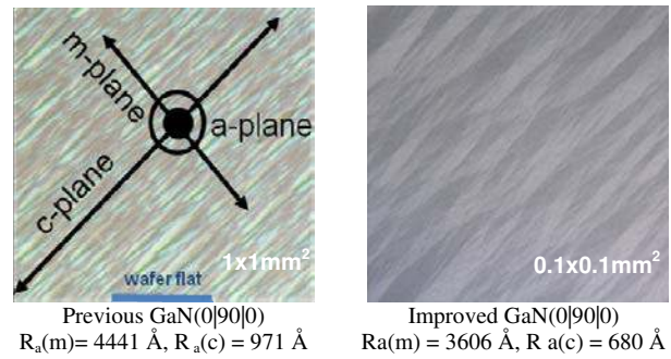
Figure 3 Surface morphology and roughness of unpolished, textured a-plane GaN (light microscope photos) of previous [6] and improved process [7].
