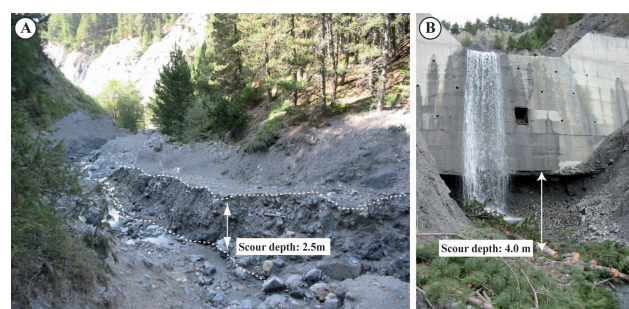
Fig. 3. Morphology of the scouring zones after the 2003 debris-flow event at the Faucon torrent. (a) View of a scoured stretch, (b) View of a strong scouring at the toe of a check dam.
