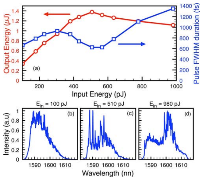
Fig. 3. (Color online) (a) Output energy of compressed pulses and corresponding FWHM duration versus energy of input pulse for the final amplifier with a pump power of 15.8 W. (b), (c), and (d) represent the spectrum of the compressed pulses for different input energies.
