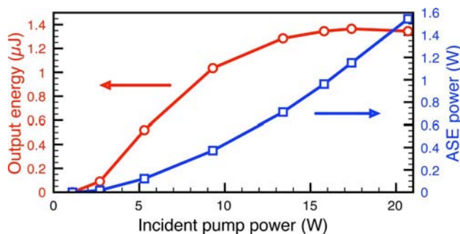
Fig. 2. (Color online) Evolution of the pulse energy after the grating compressor and the ASE power generated by the power amplifier versus pump power and for input pulse energy of 500 pJ.
